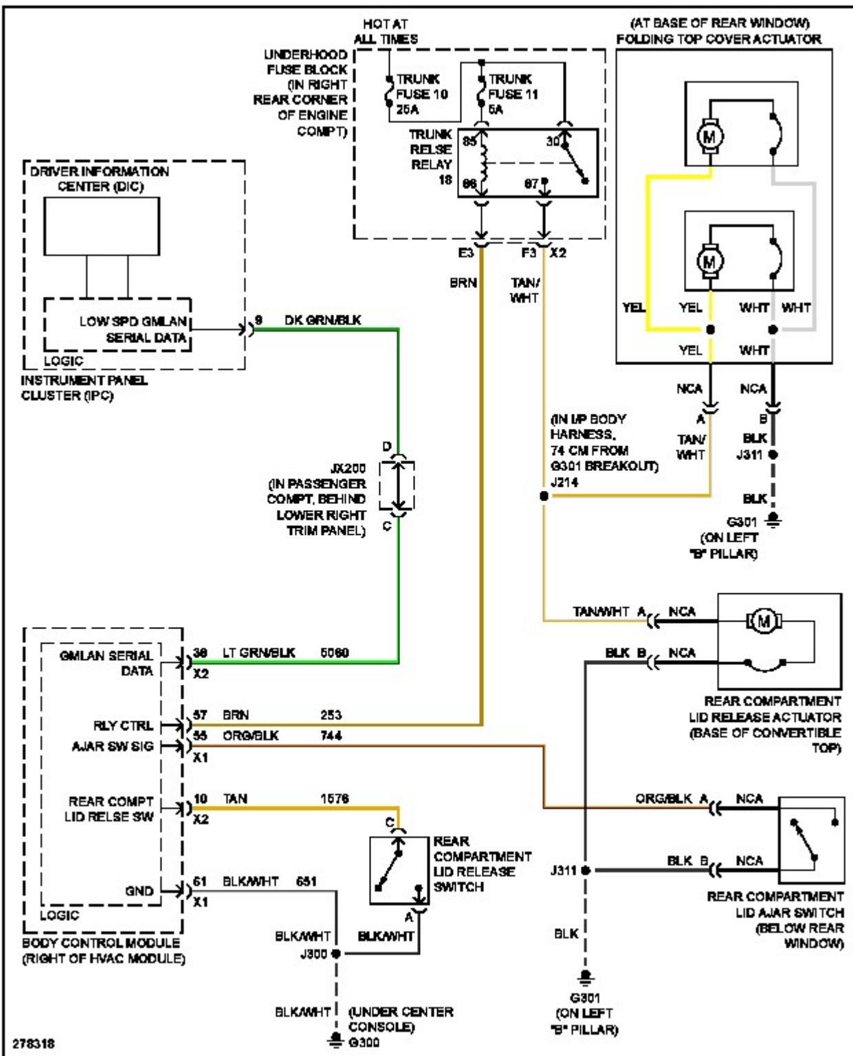
Fig. 54: Trunk Release Circuit
