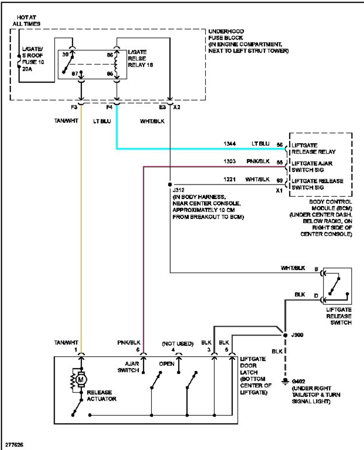
Fig. 59: Liftgate Release Circuit
